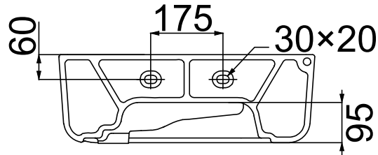
BACK VIEW
